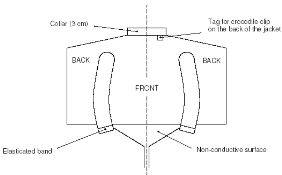
Figure 15. Electric sabre: conductive jacket
