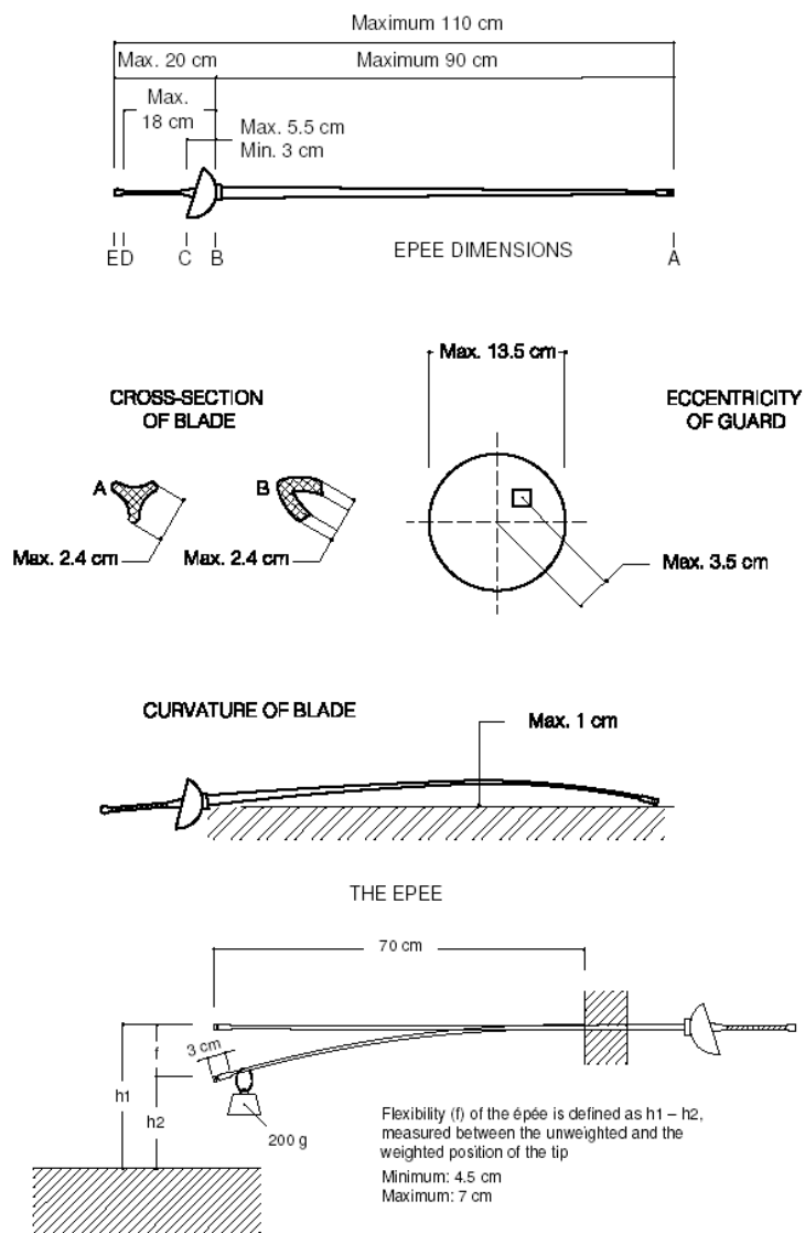
Figure 9. Epee dimensions and flexibility
